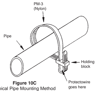
Typical Pipe Mounting Method
